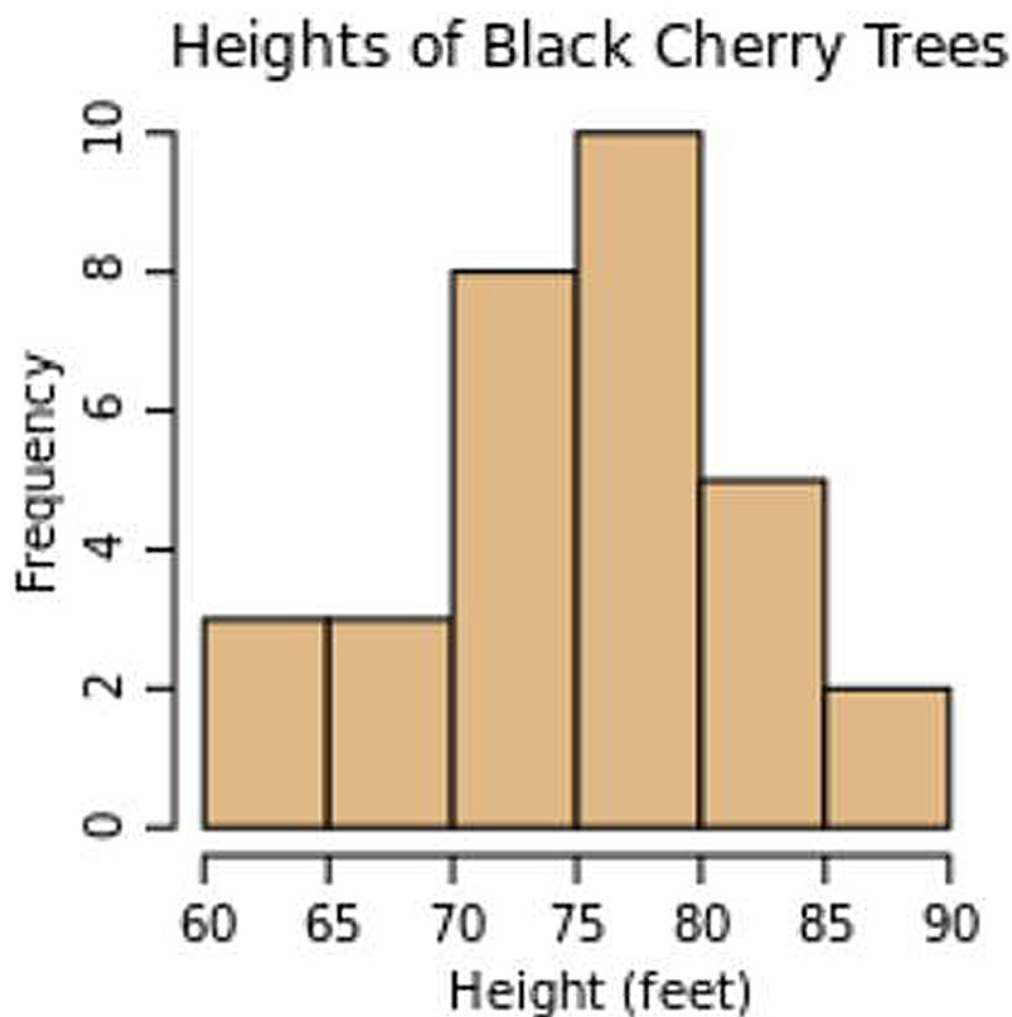
Figure 3: Histogram example
